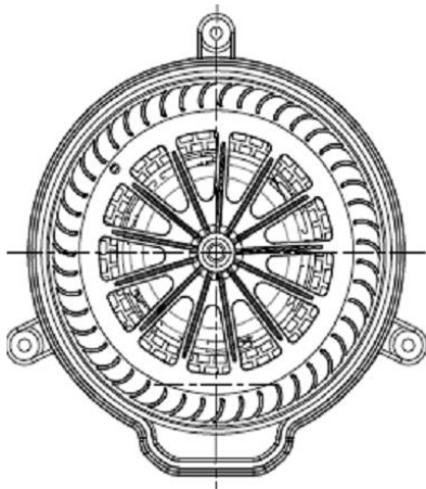
INLET VIEW
